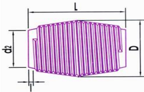
圆锥形接头尺寸图 Dimension drawing of conical nipples
